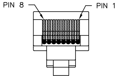
SECTION A-A END VIEW 8P8C, RJ45 PLUG
