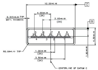
USB 3.0 Standard-A Plug Pin Assignment
